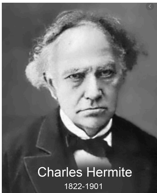
The French mathematician Charles Hermite.#
