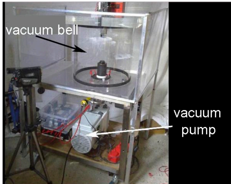
J.P.Petit's makeshift laboratory
