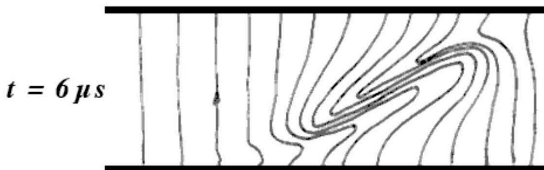
Distortion of the electric current lines by the electrothermal instability of Velikhov
