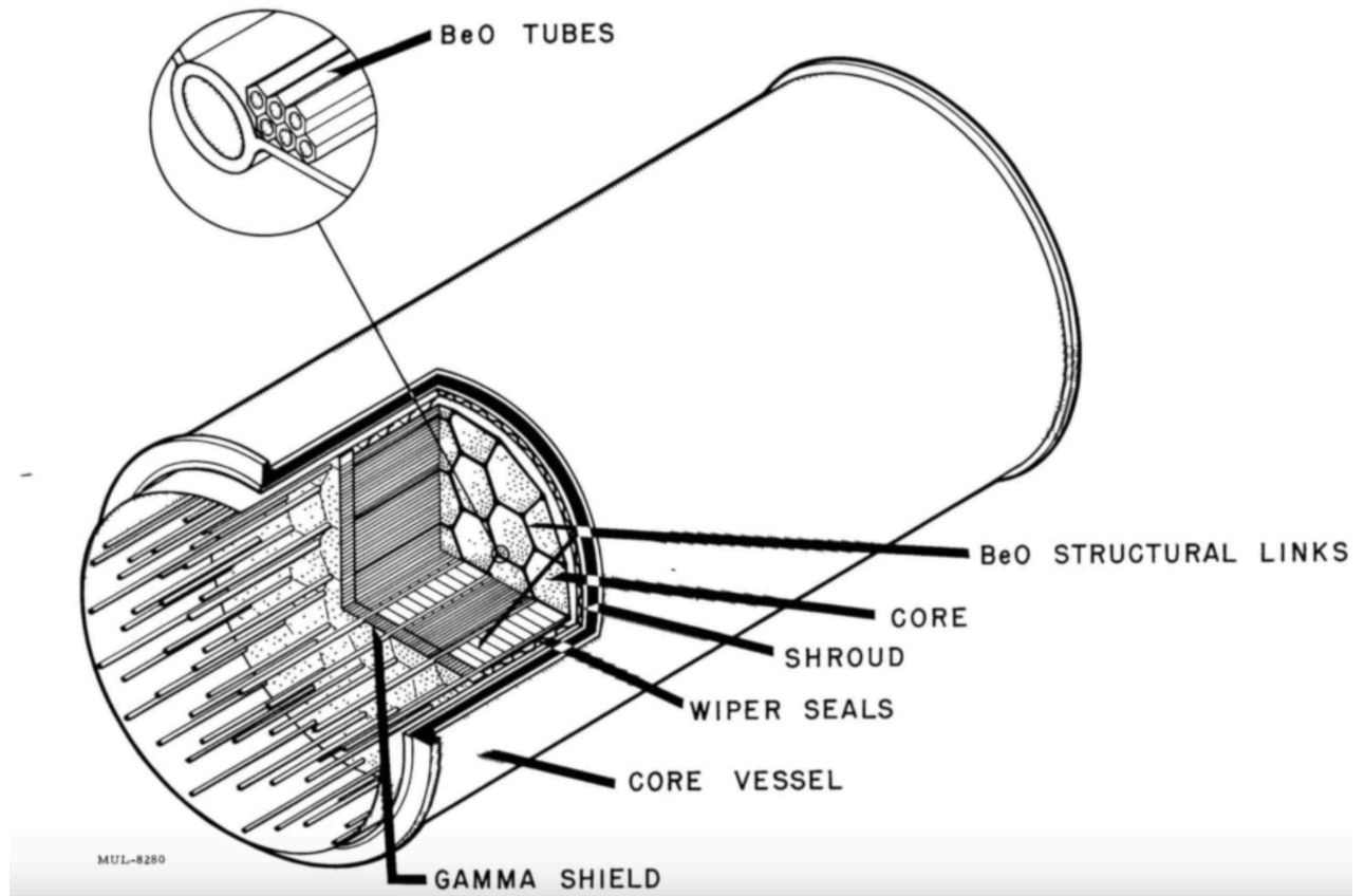
The nuclear engine of Pluto
