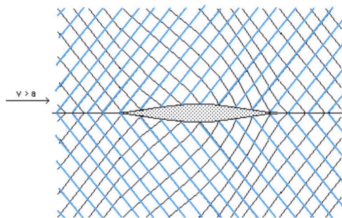
Fig.5 Mach lines from action of the \mathbf{J} \times \mathbf{B} force field
