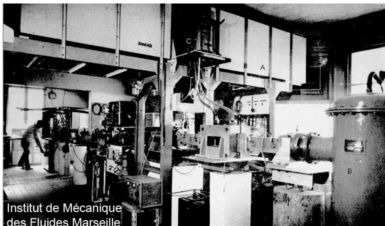
Jean-Pierre Petit's hot shock driven wind tunnel, in 1965.
